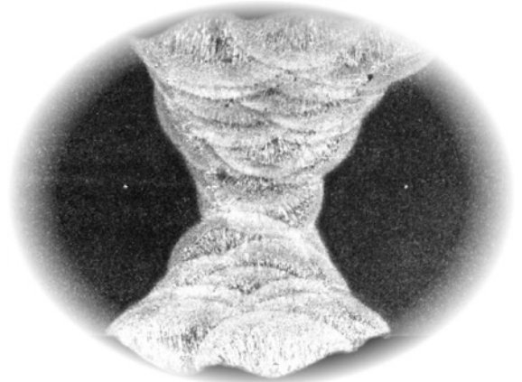
Macro photograph of a wet-weld at x3 magnification
